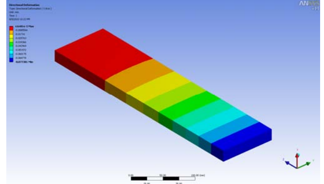
Figure 2. Ansys simulation showing deflection
