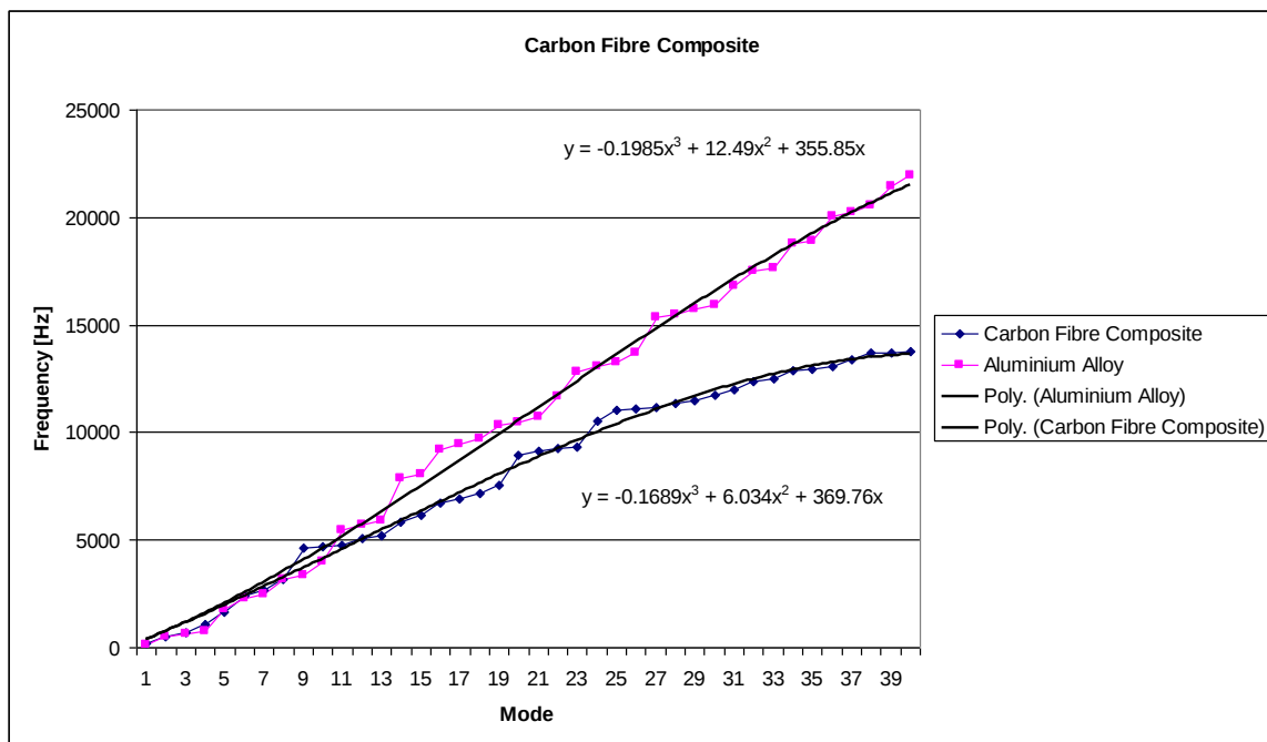
Fig. 2: Modal analysis results.
